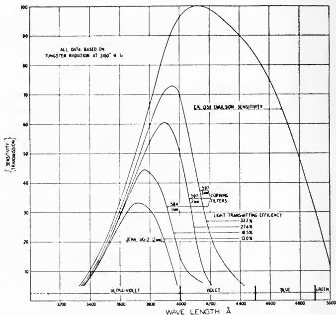
FIG. 2. Sensitivity of sound negative emulsion and transmission characteristics of filters. Based on tungsten light at 3000°K.
